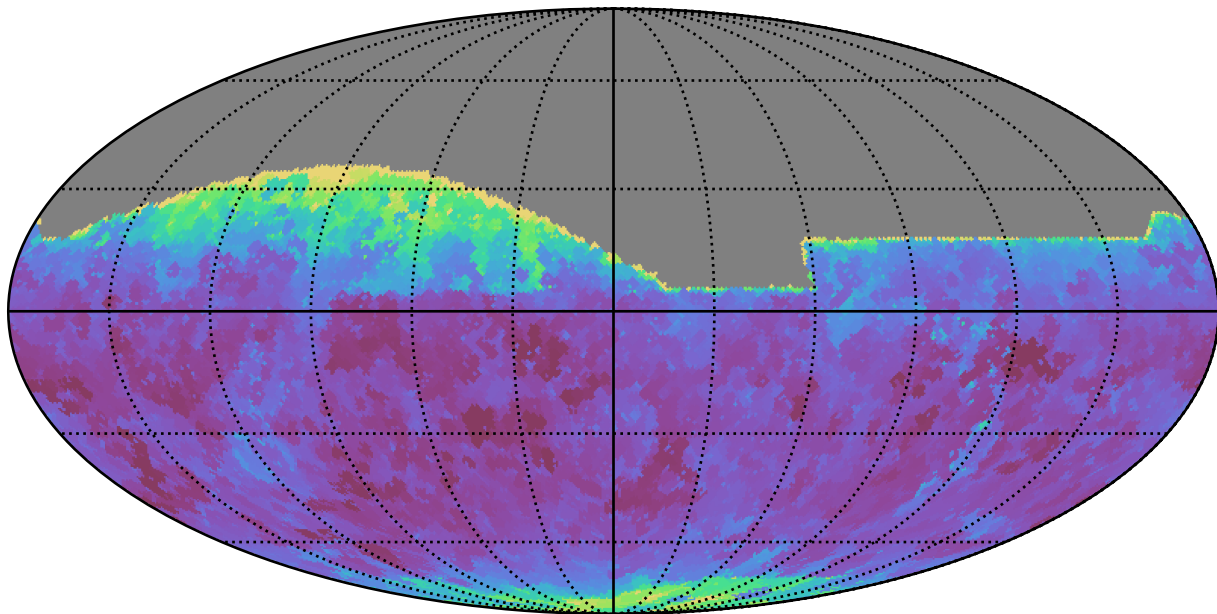
ddf_loaded_fl1_v3.4_10yrs All sky z band: Min seeingEff
