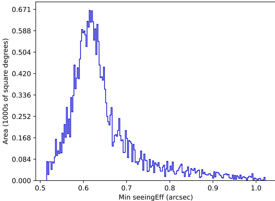
ddf_loaded_fl1_v3.4_10yrs All sky z band: Min seeingEff
