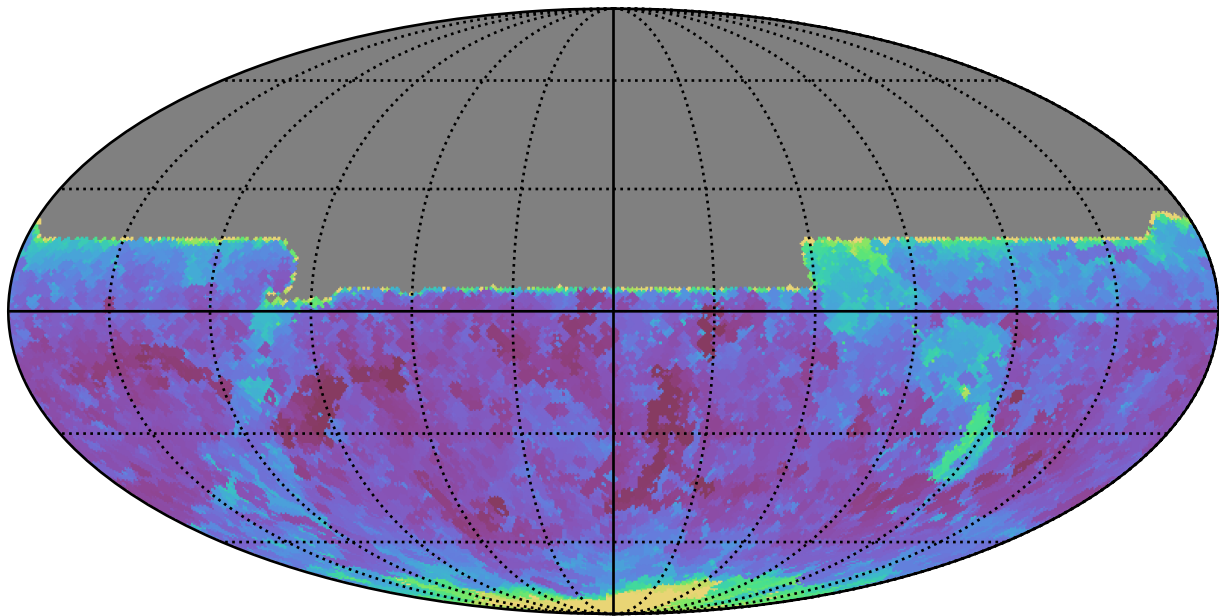
ddf_loaded_fl1_v3.4_10yrs All sky y band: Min seeingEff
