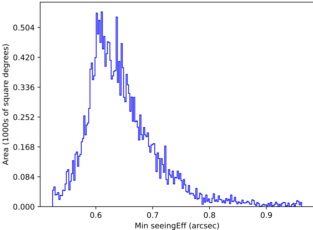
ddf_loaded_fl1_v3.4_10yrs All sky y band: Min seeingEff
