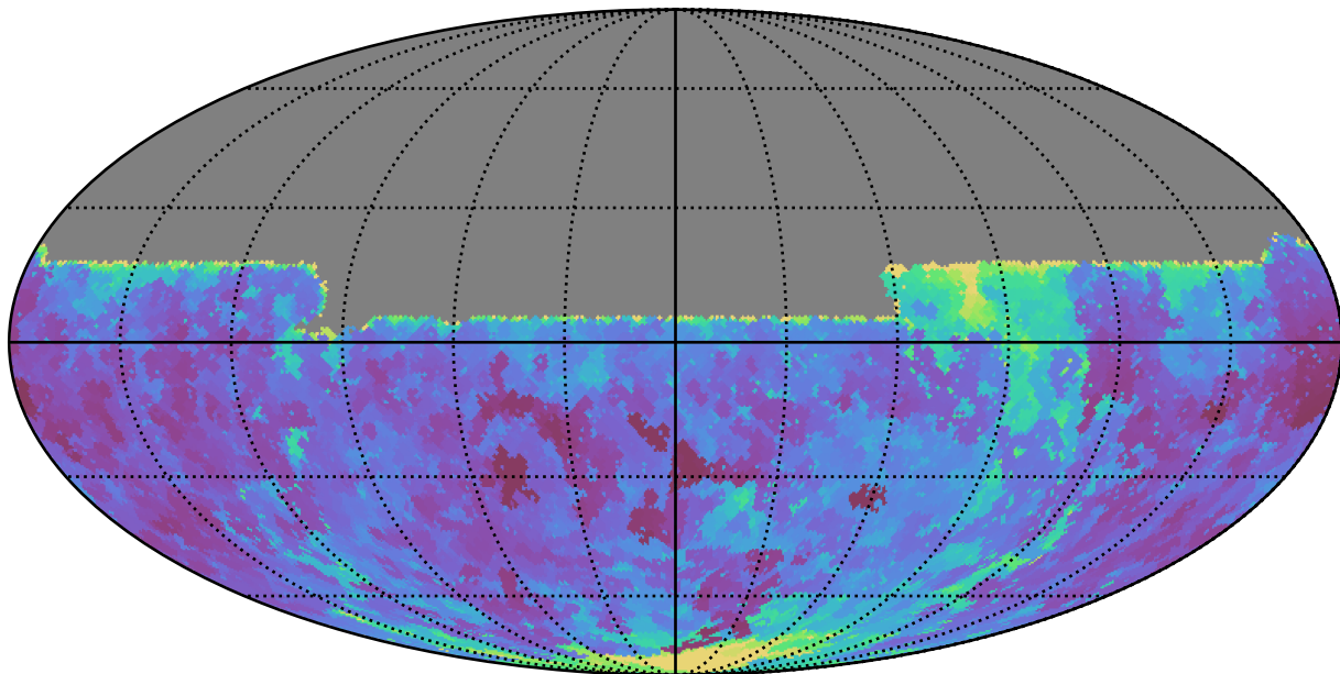
ddf_loaded_fl1_v3.4_10yrs All sky u band: Min seeingEff
