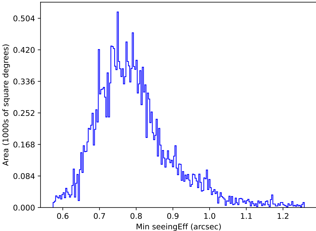
ddf_loaded_fl1_v3.4_10yrs All sky u band: Min seeingEff
