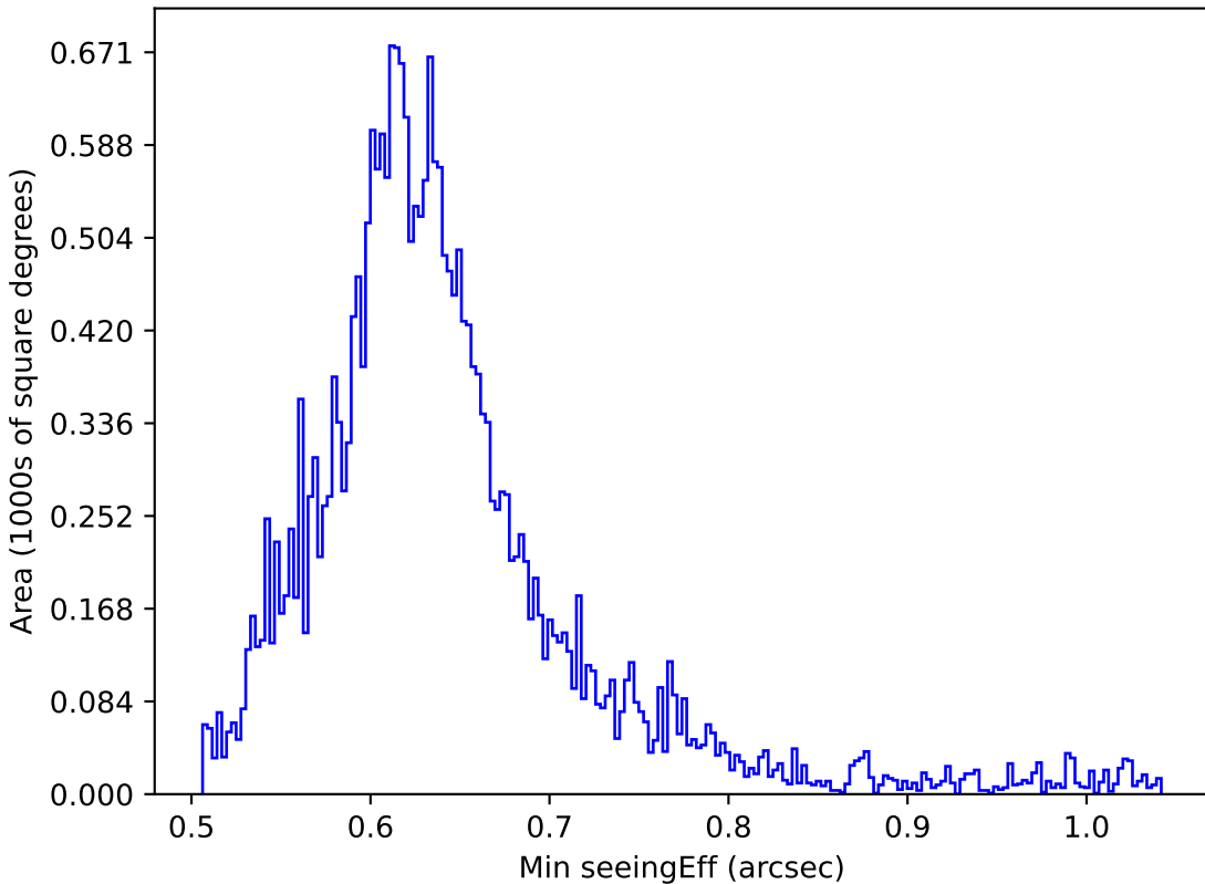
ddf_loaded_fl1_v3.4_10yrs All sky r band: Min seeingEff
