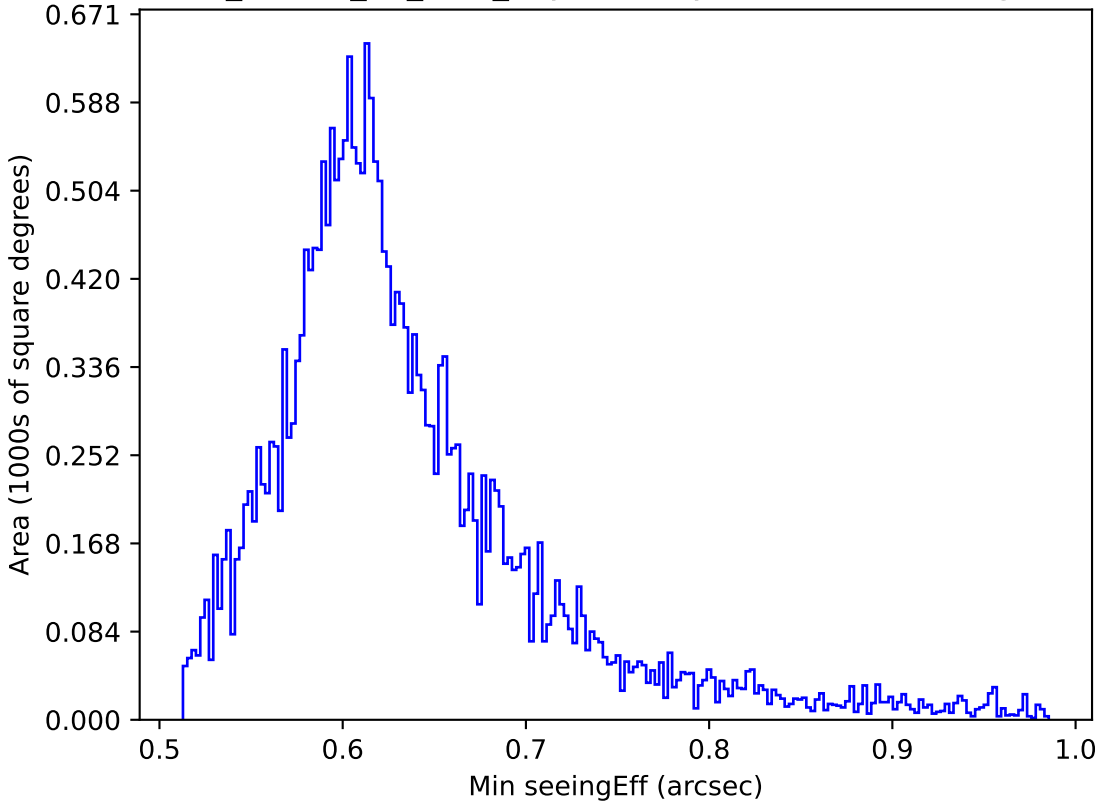
ddf_loaded_fl1_v3.4_10yrs All sky i band: Min seeingEff
