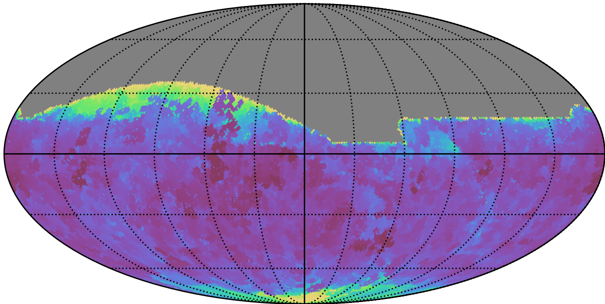
ddf_loaded_fl1_v3.4_10yrs All sky g band: Min seeingEff
