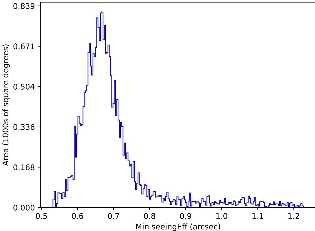
ddf_loaded_fl1_v3.4_10yrs All sky g band: Min seeingEff
