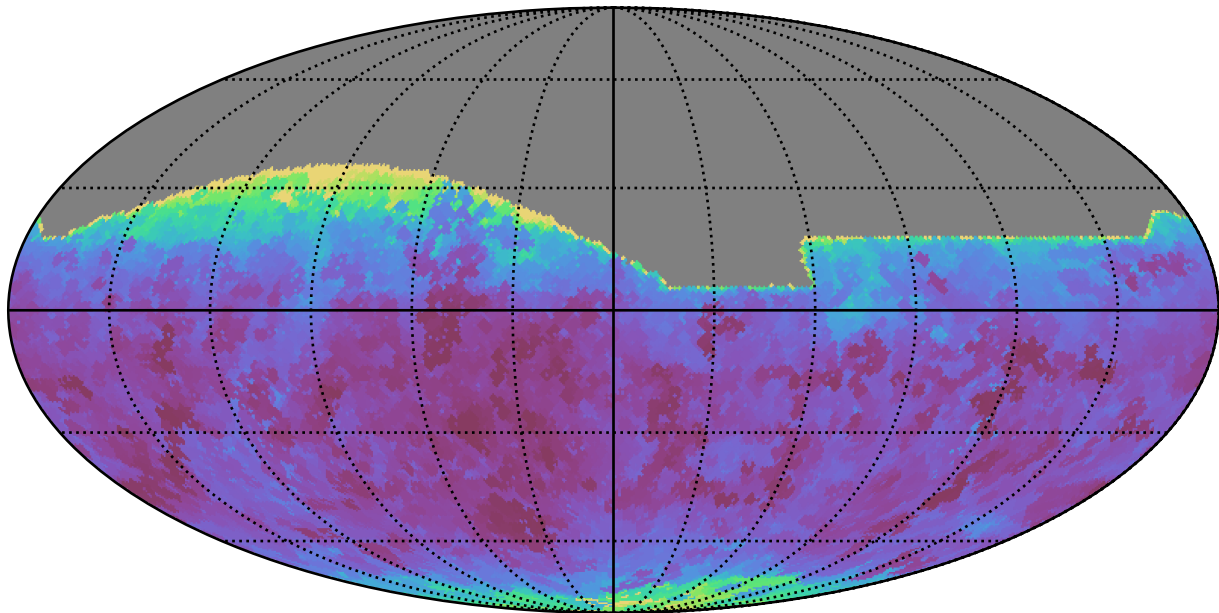
ddf_loaded_fl1_v3.4_10yrs All sky all bands: Min seeingEff
