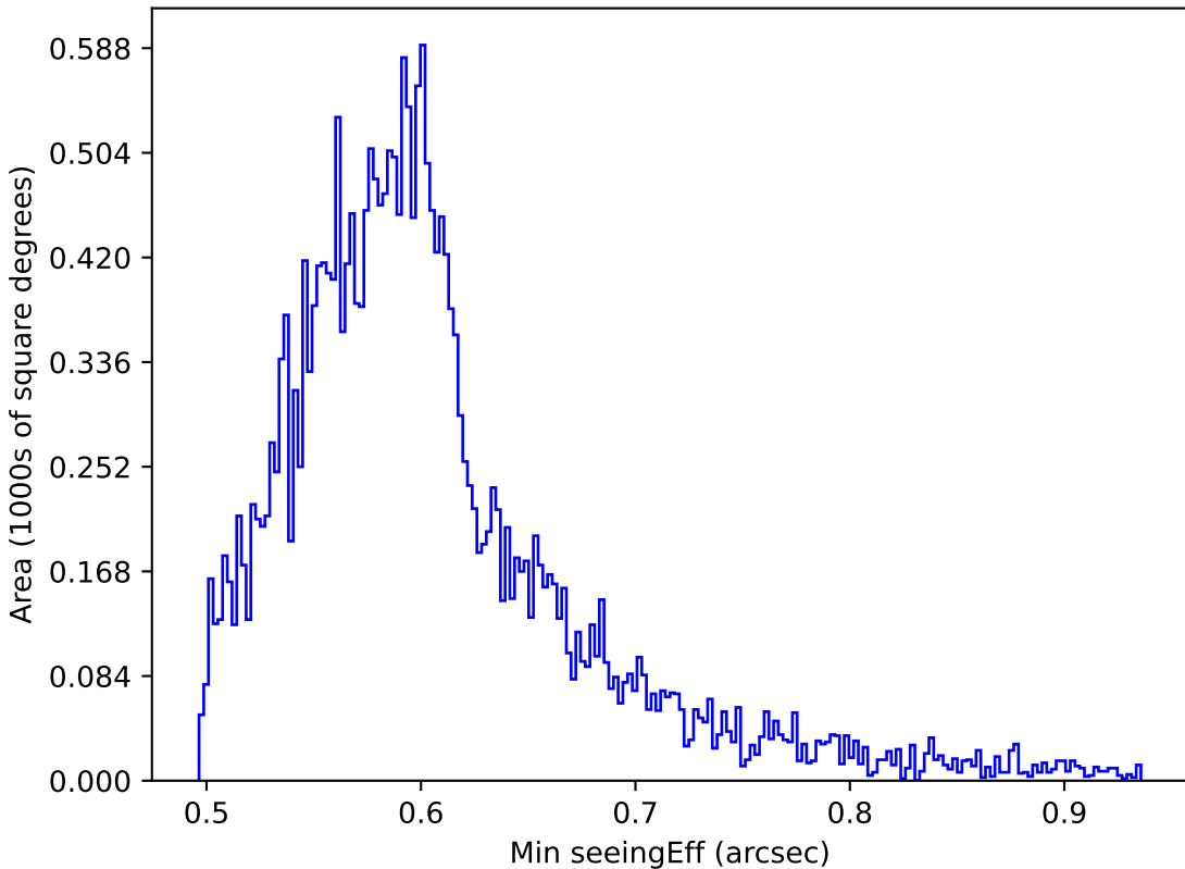
ddf_loaded_fl1_v3.4_10yrs All sky all bands: Min seeingEff
