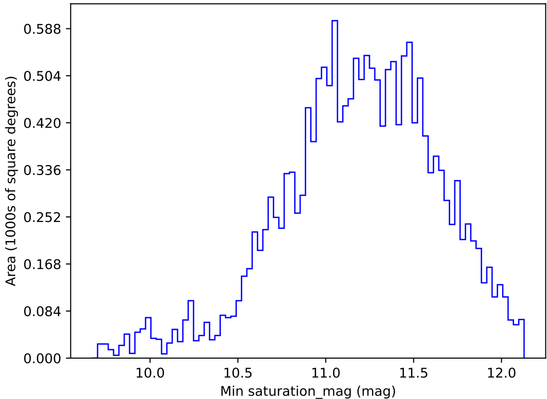
ddf_loaded_fl1_v3.4_10yrs WFD y band: Min saturation_mag
