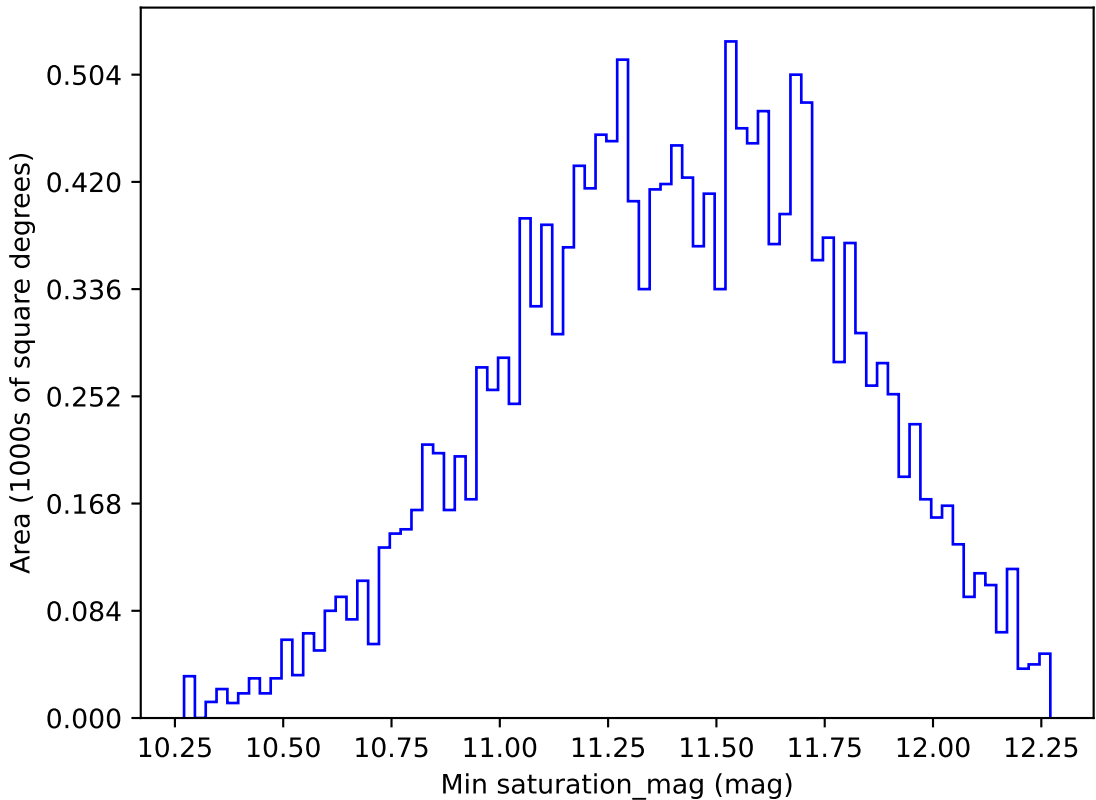
ddf_loaded_fl1_v3.4_10yrs WFD u band: Min saturation_mag
