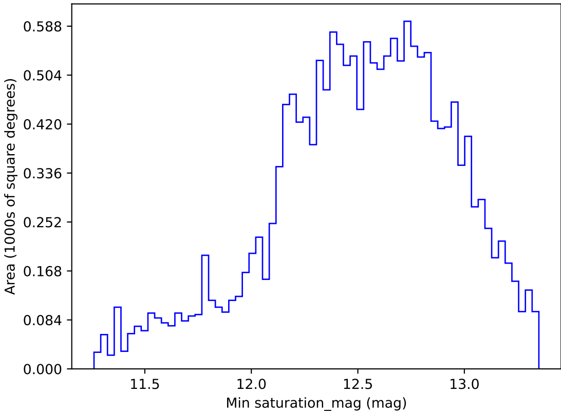
ddf_loaded_fl1_v3.4_10yrs WFD r band: Min saturation_mag
