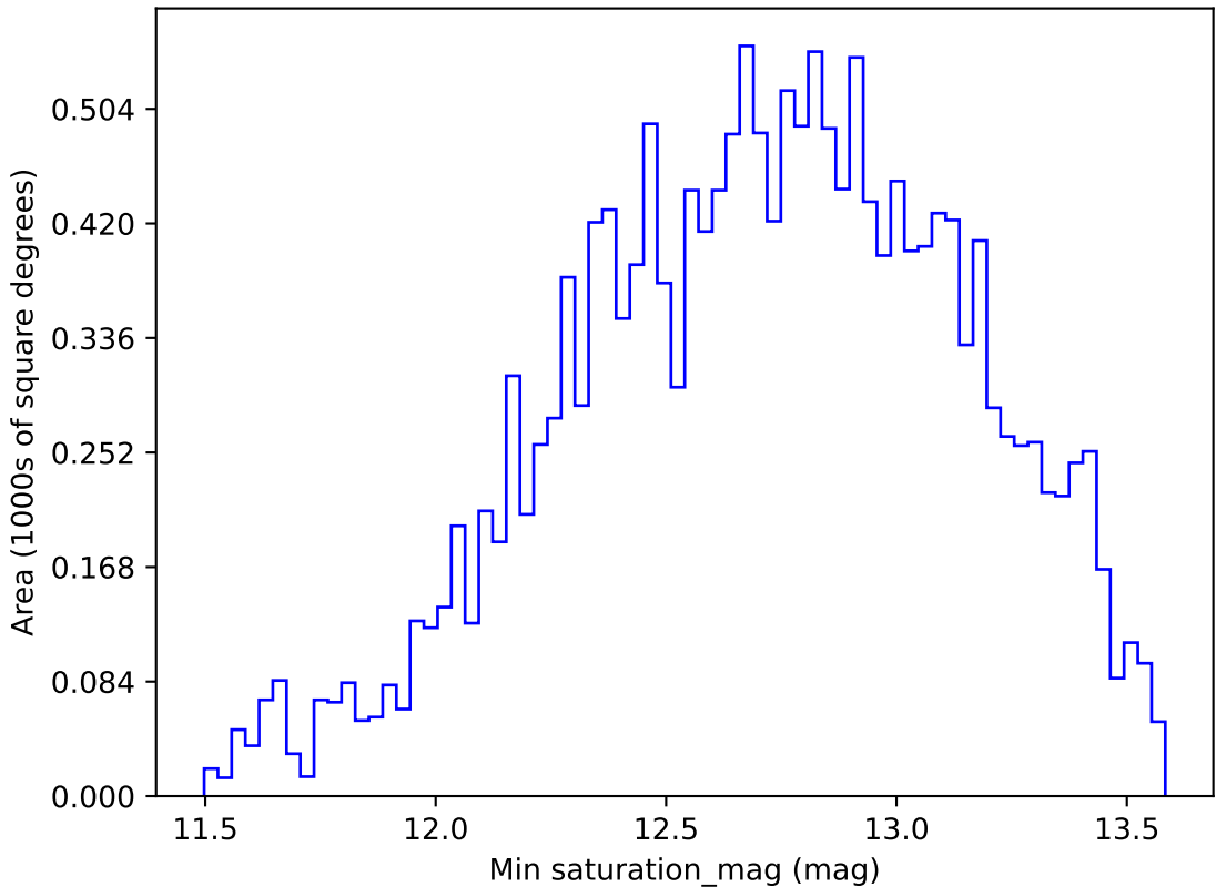
ddf_loaded_fl1_v3.4_10yrs WFD g band: Min saturation_mag
