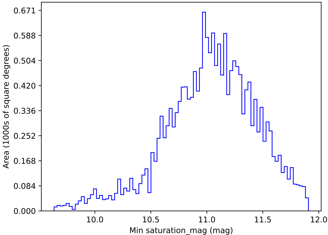
ddf_loaded_fl1_v3.4_10yrs WFD all bands: Min saturation_mag
