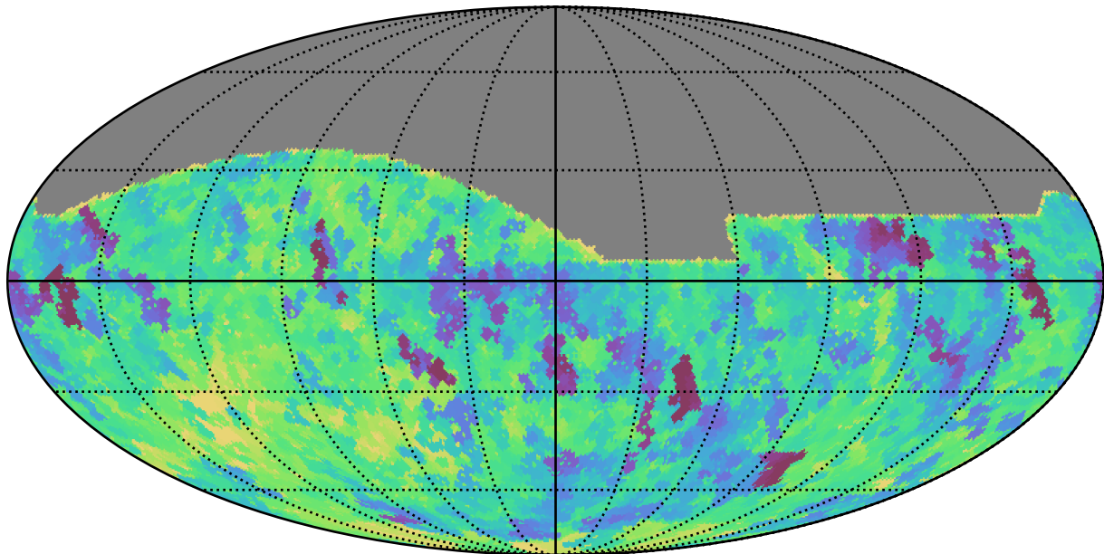
ddf_loaded_fl1_v3.4_10yrs All sky z band: Min saturation_mag
