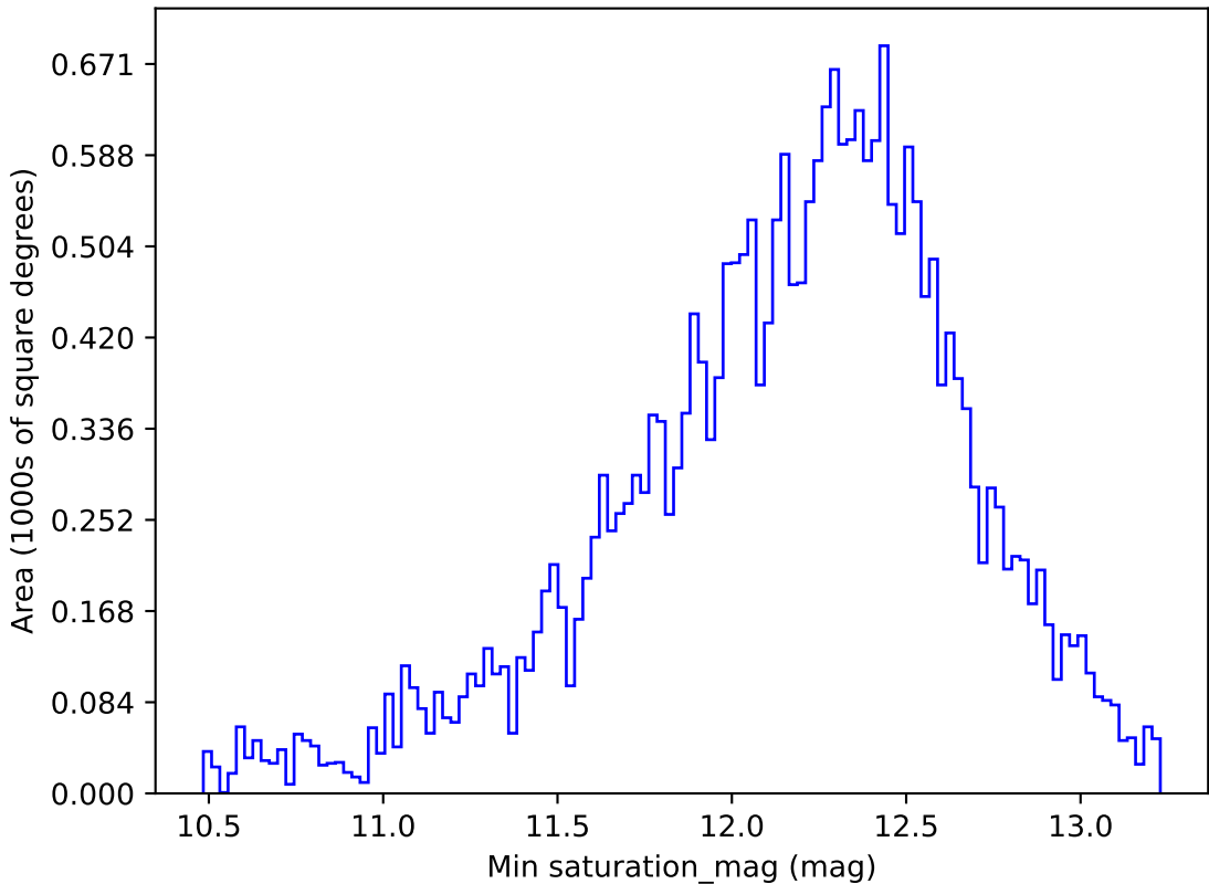
ddf_loaded_fl1_v3.4_10yrs All sky z band: Min saturation_mag
