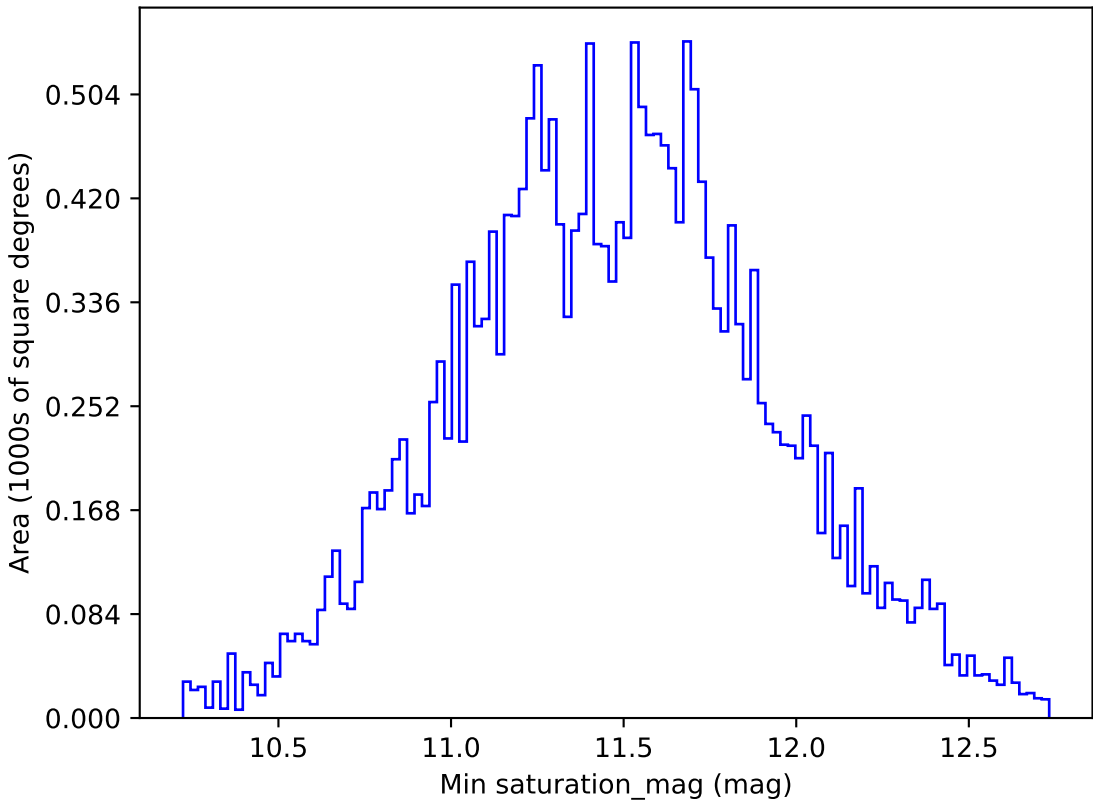
ddf_loaded_fl1_v3.4_10yrs All sky u band: Min saturation_mag
