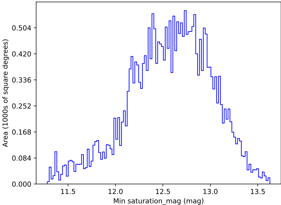
ddf_loaded_fl1_v3.4_10yrs All sky r band: Min saturation_mag
