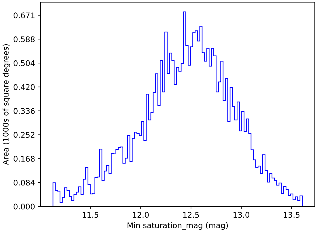
ddf_loaded_fl1_v3.4_10yrs All sky i band: Min saturation_mag
