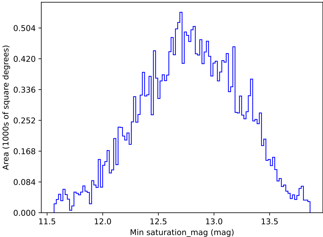
ddf_loaded_fl1_v3.4_10yrs All sky g band: Min saturation_mag
