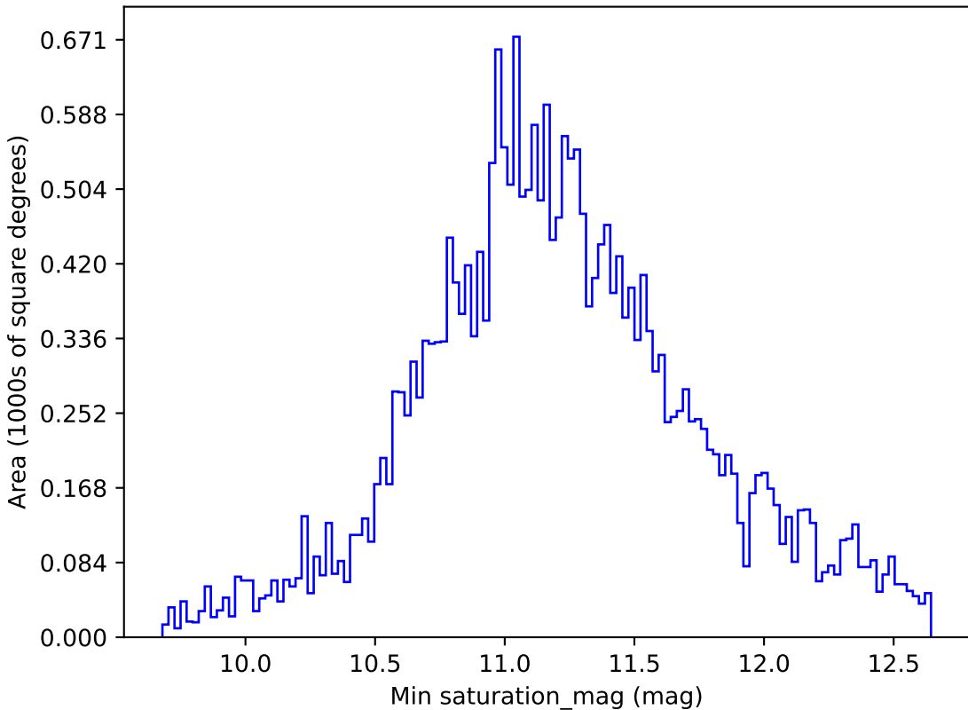
ddf_loaded_fl1_v3.4_10yrs All sky all bands: Min saturation_mag
