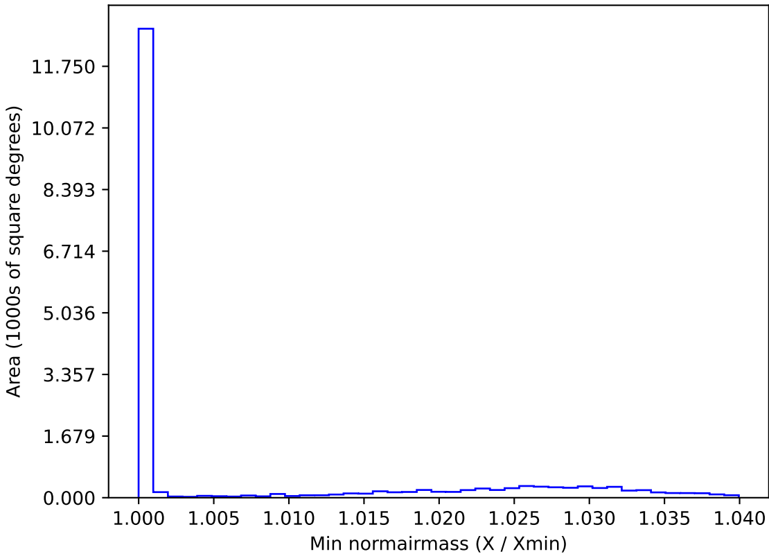
ddf_loaded_fl1_v3.4_10yrs WFD y band: Min normairmass
