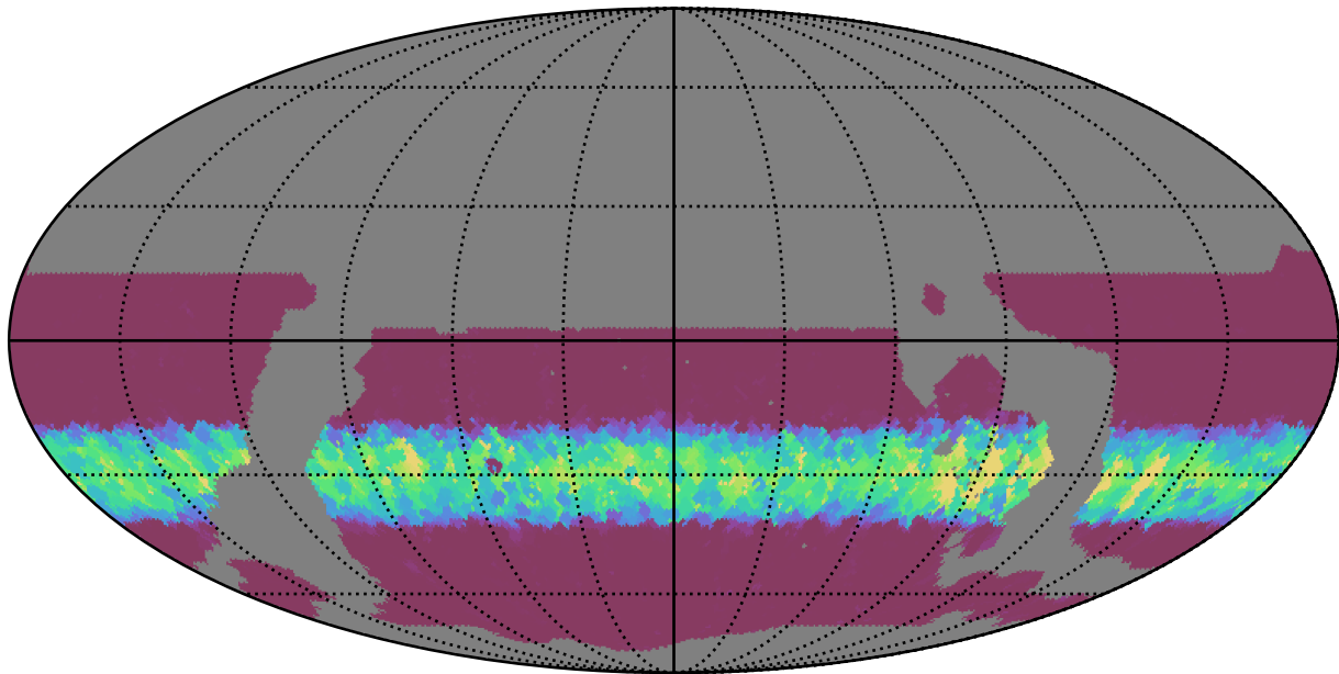
ddf_loaded_fl1_v3.4_10yrs WFD u band: Min normairmass
