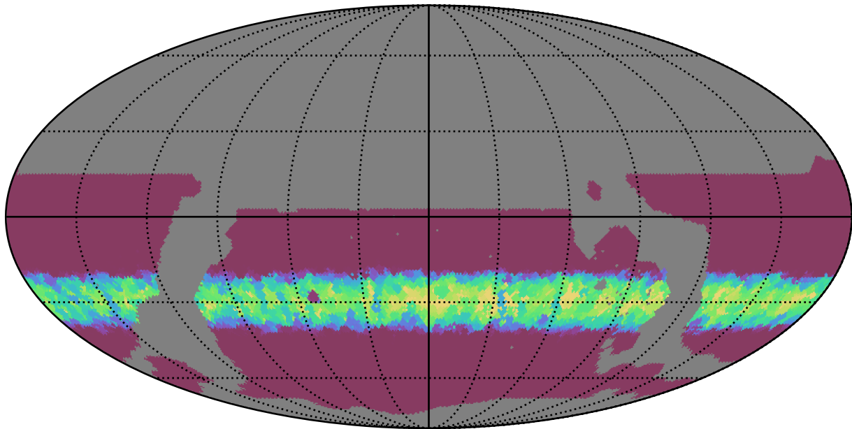
ddf_loaded_fl1_v3.4_10yrs WFD r band: Min normairmass
