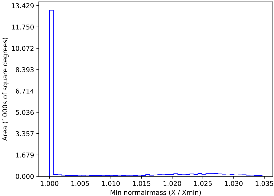
ddf_loaded_fl1_v3.4_10yrs WFD r band: Min normairmass
