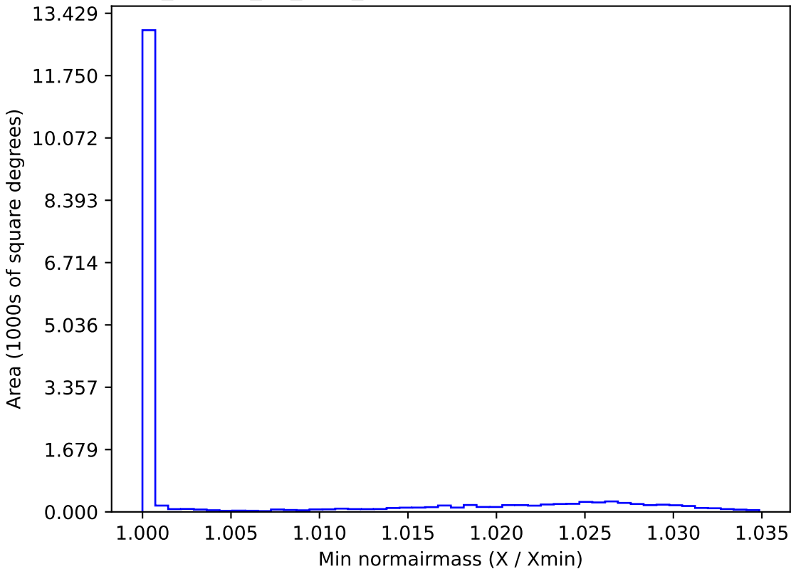
ddf_loaded_fl1_v3.4_10yrs WFD i band: Min normairmass
