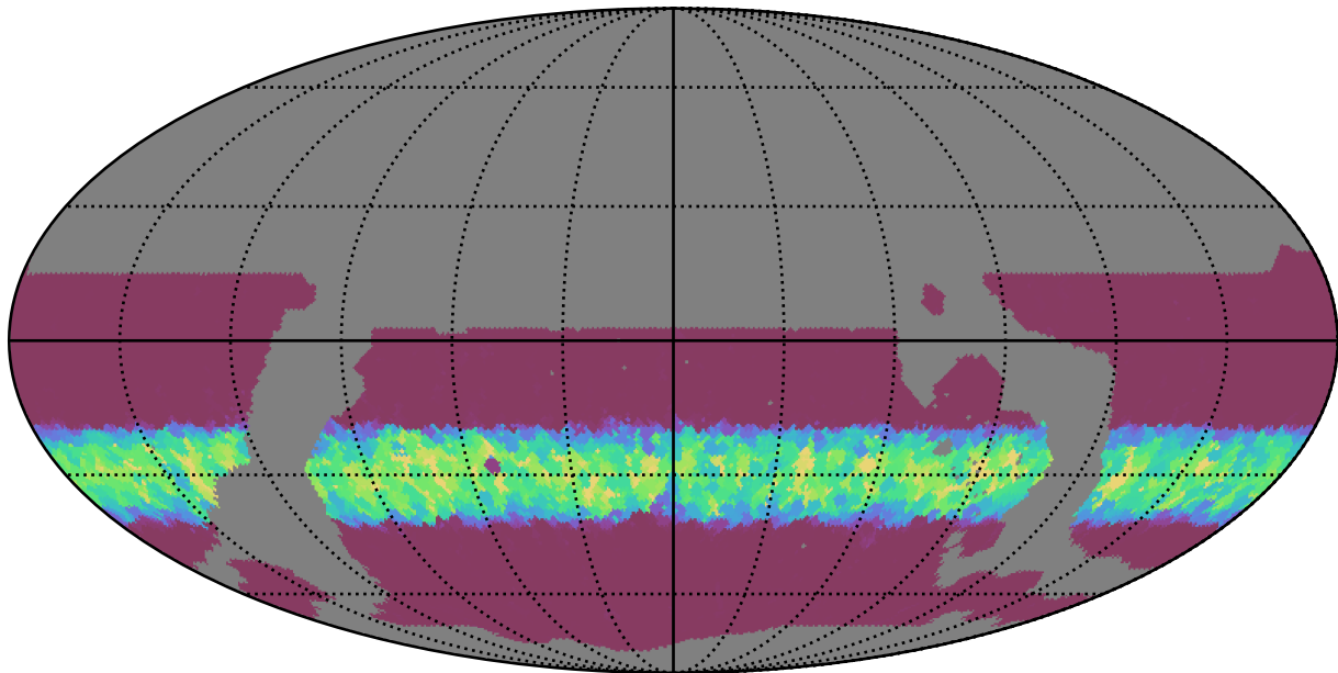
ddf_loaded_fl1_v3.4_10yrs WFD g band: Min normairmass
