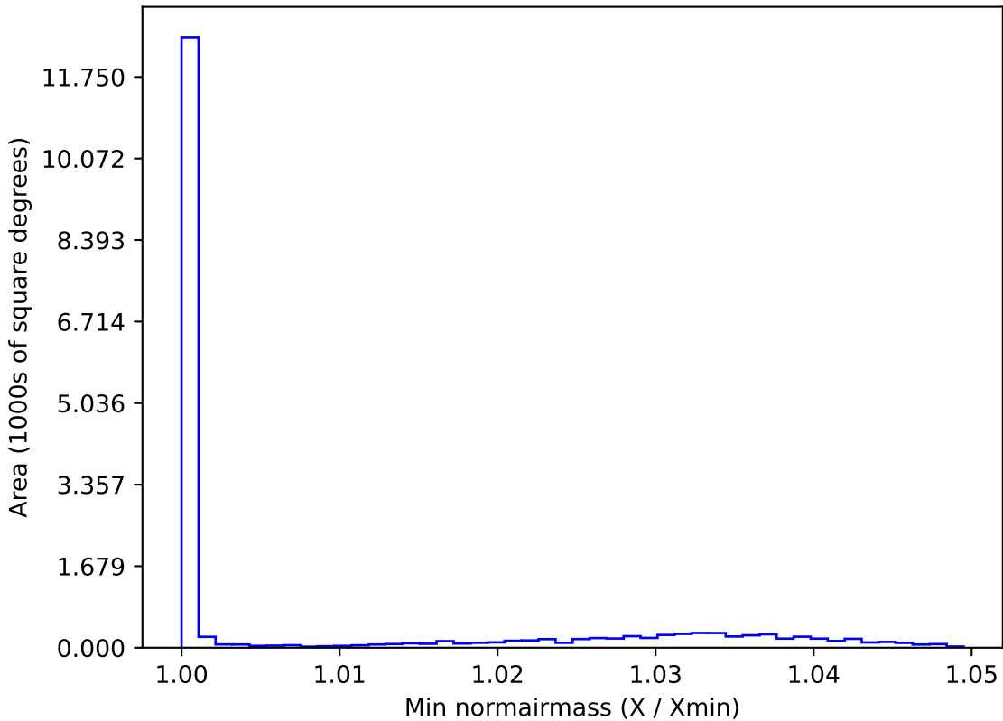
ddf_loaded_fl1_v3.4_10yrs WFD g band: Min normairmass
