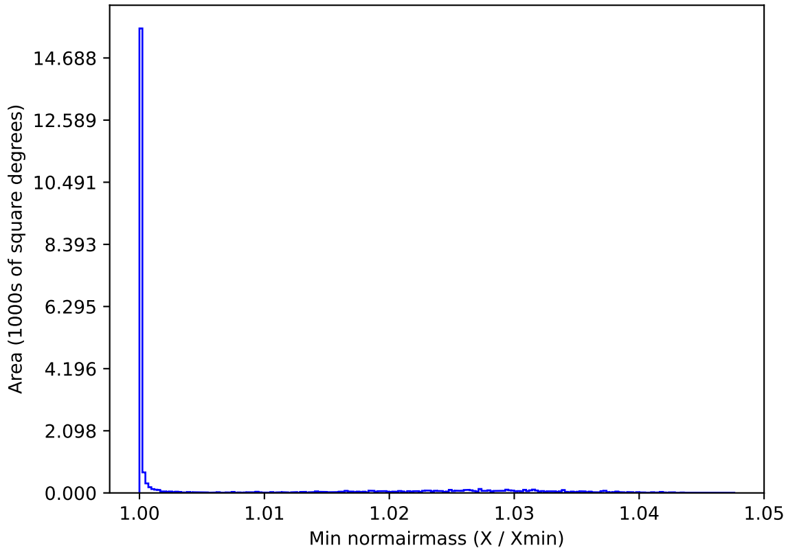
ddf_loaded_fl1_v3.4_10yrs All sky y band: Min normairmass
