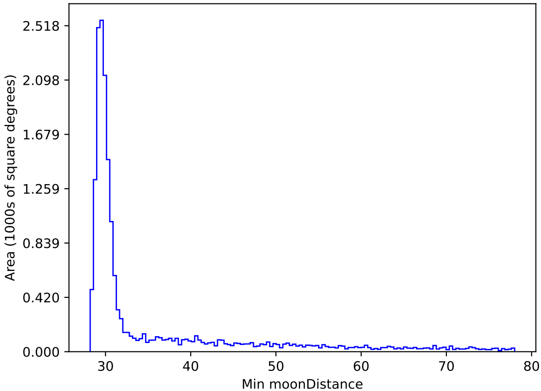
ddf_loaded_fl1_v3.4_10yrs WFD z band: Min moonDistance
