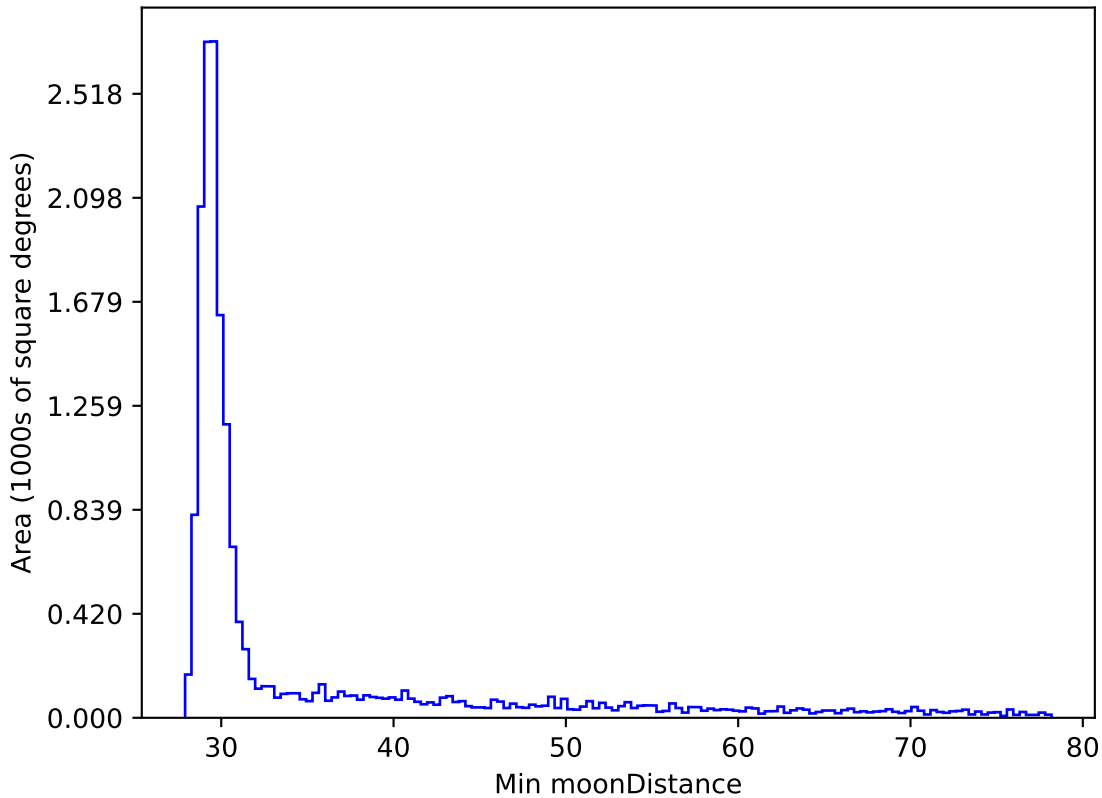
ddf_loaded_fl1_v3.4_10yrs WFD y band: Min moonDistance
