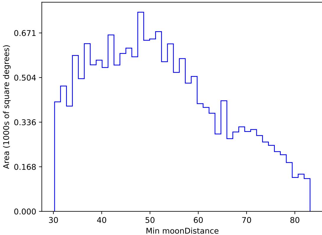
ddf_loaded_fl1_v3.4_10yrs WFD u band: Min moonDistance
