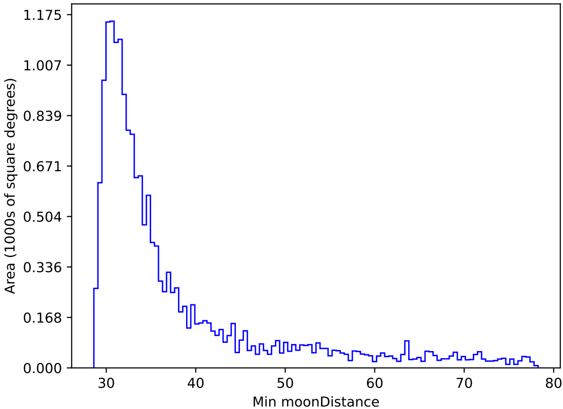
ddf_loaded_fl1_v3.4_10yrs WFD r band: Min moonDistance
