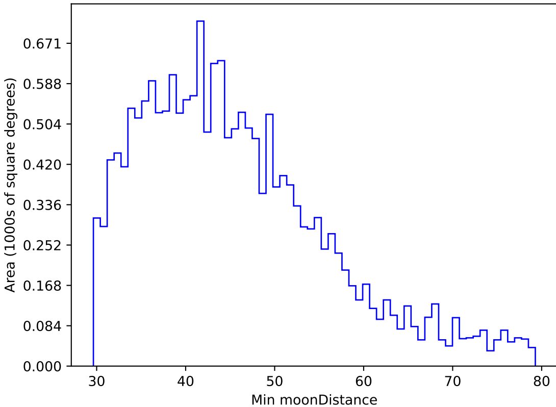
ddf_loaded_fl1_v3.4_10yrs WFD g band: Min moonDistance
