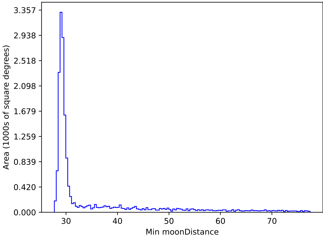
ddf_loaded_fl1_v3.4_10yrs WFD all bands: Min moonDistance
