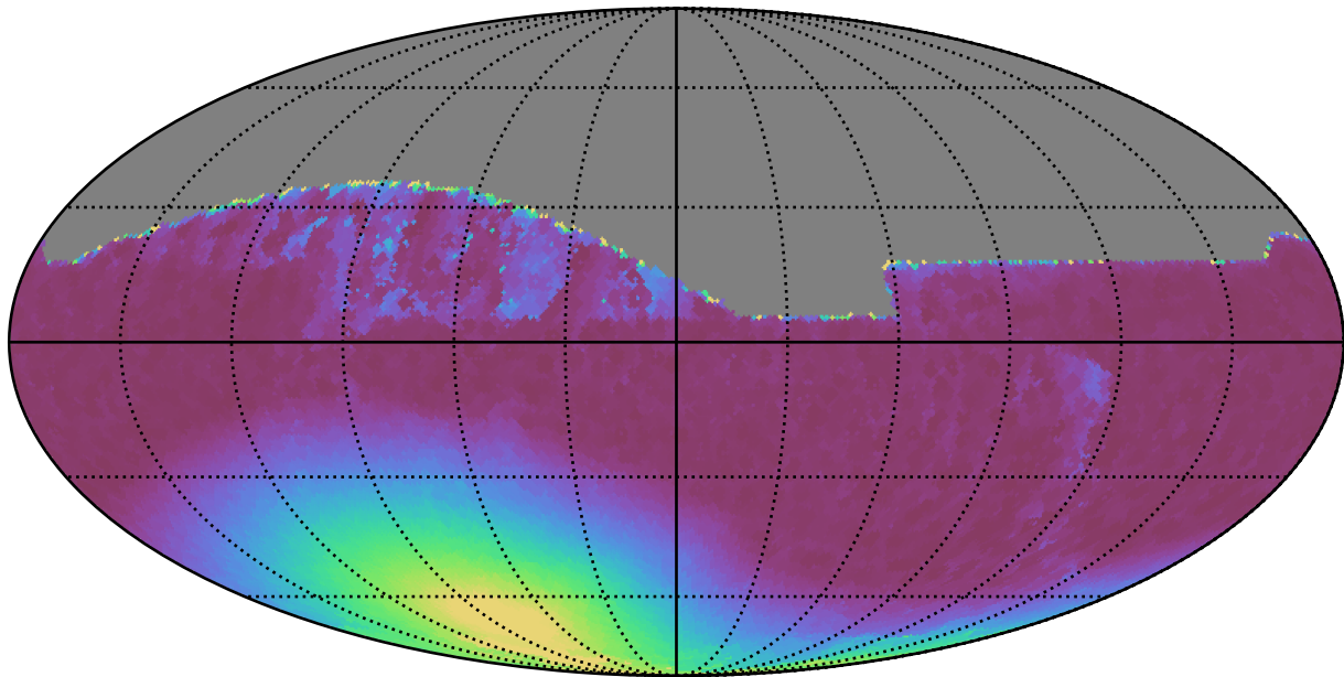
ddf_loaded_fl1_v3.4_10yrs All sky z band: Min moonDistance
