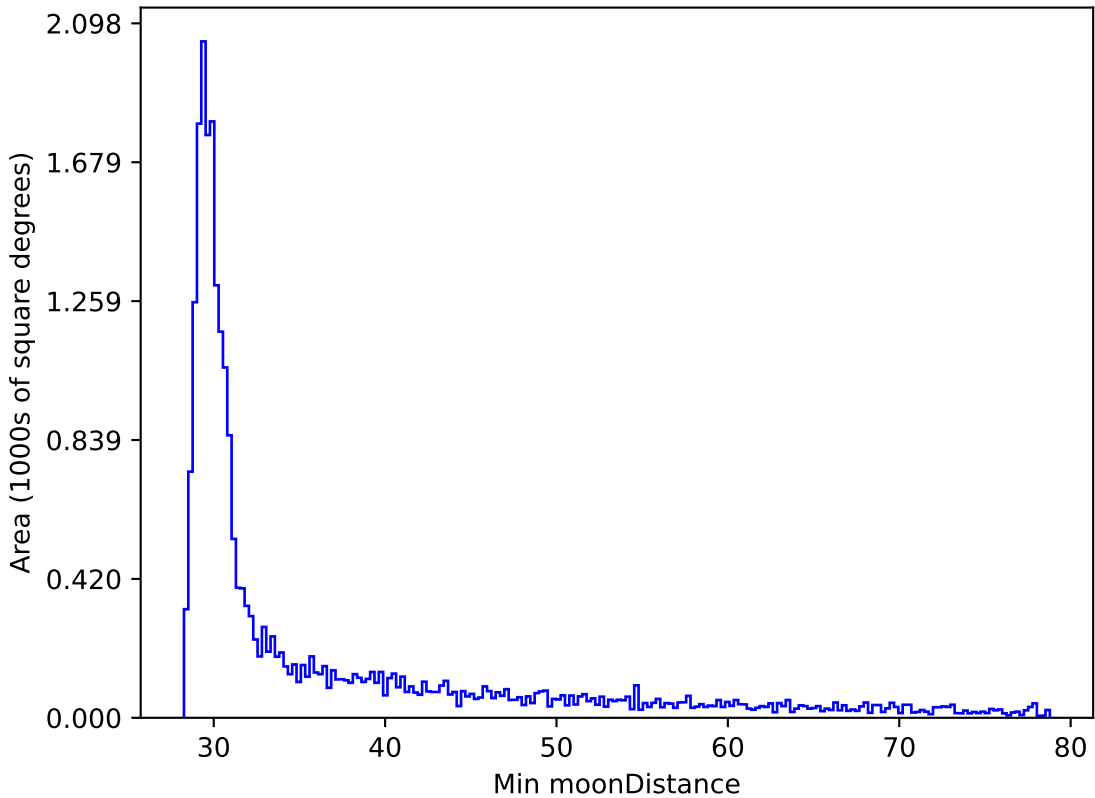
ddf_loaded_fl1_v3.4_10yrs All sky z band: Min moonDistance
