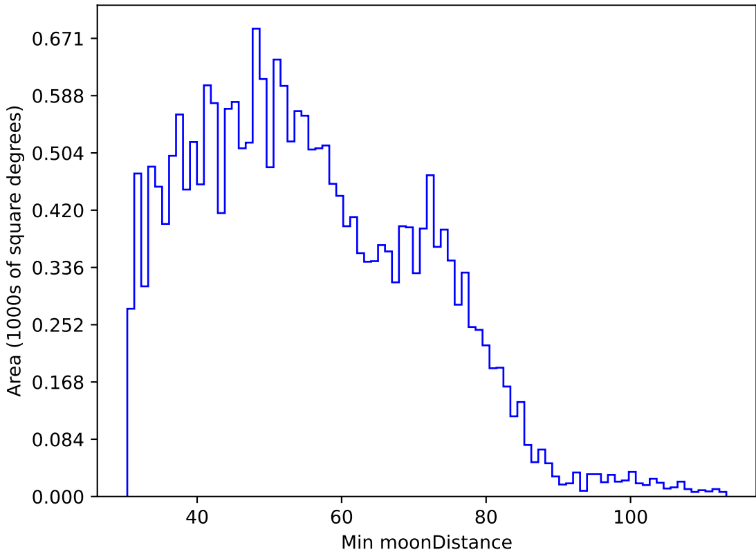
ddf_loaded_fl1_v3.4_10yrs All sky u band: Min moonDistance
