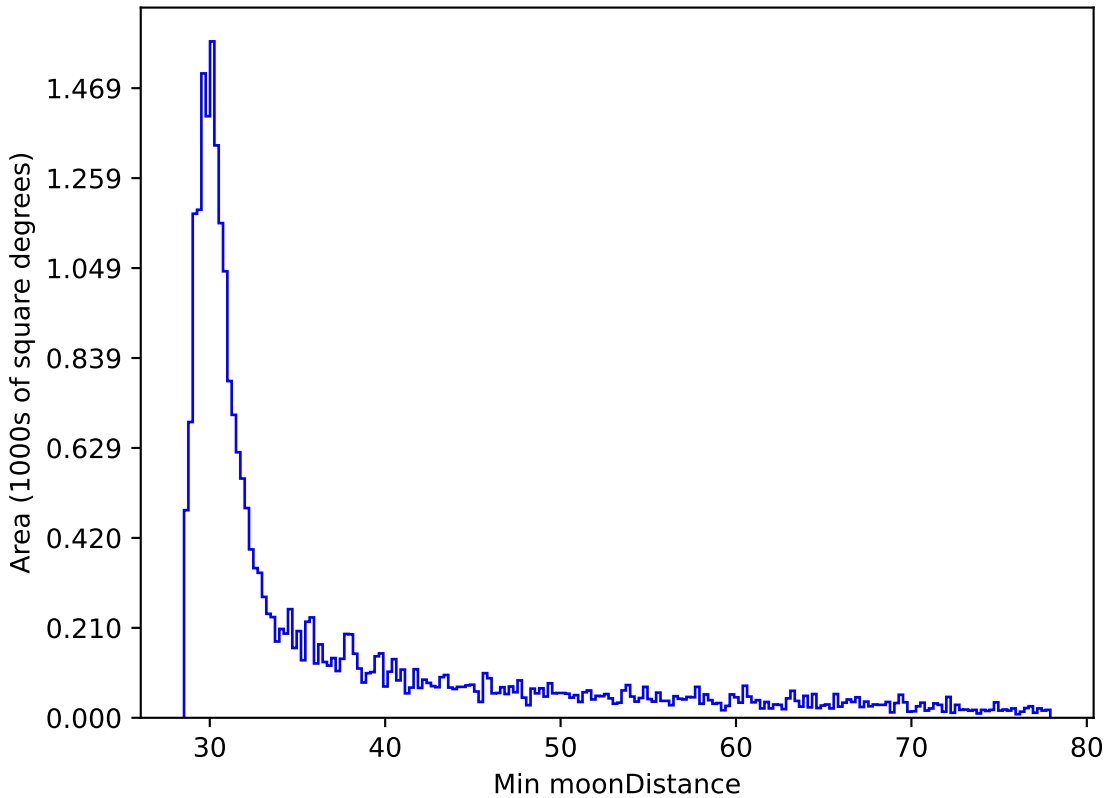
ddf_loaded_fl1_v3.4_10yrs All sky i band: Min moonDistance
