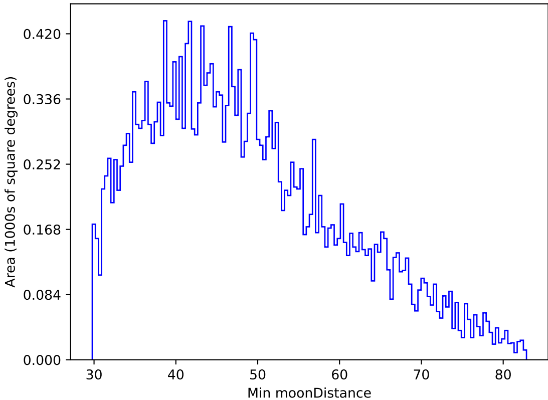
ddf_loaded_fl1_v3.4_10yrs All sky g band: Min moonDistance
