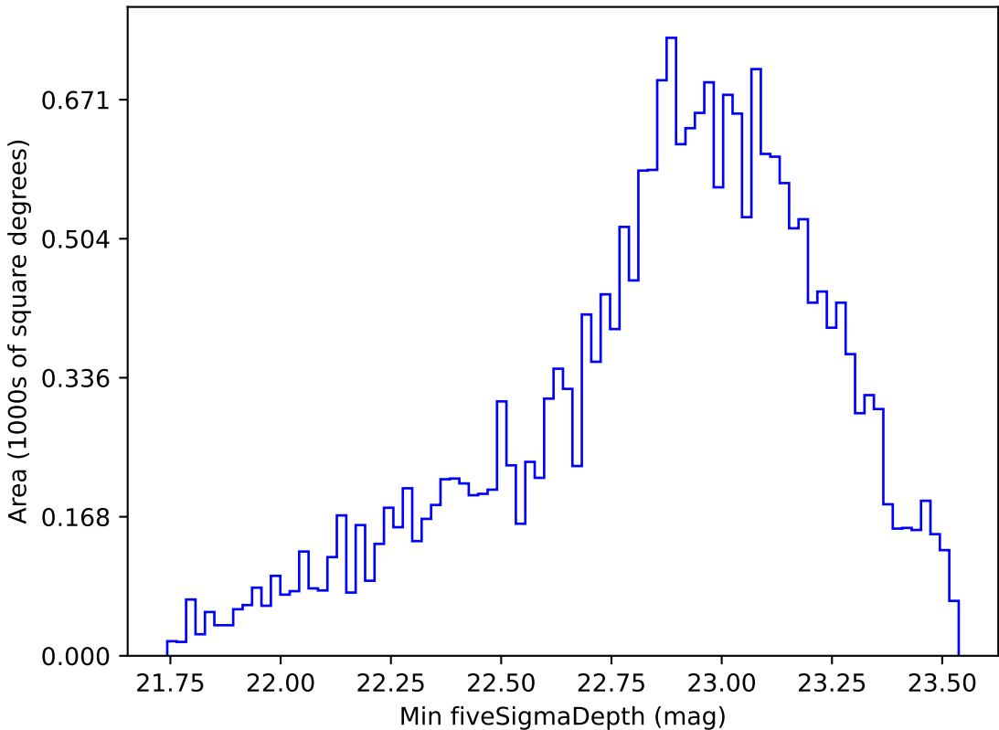
ddf_loaded_fl1_v3.4_10yrs Yr 1 u band: Min fiveSigmaDepth
