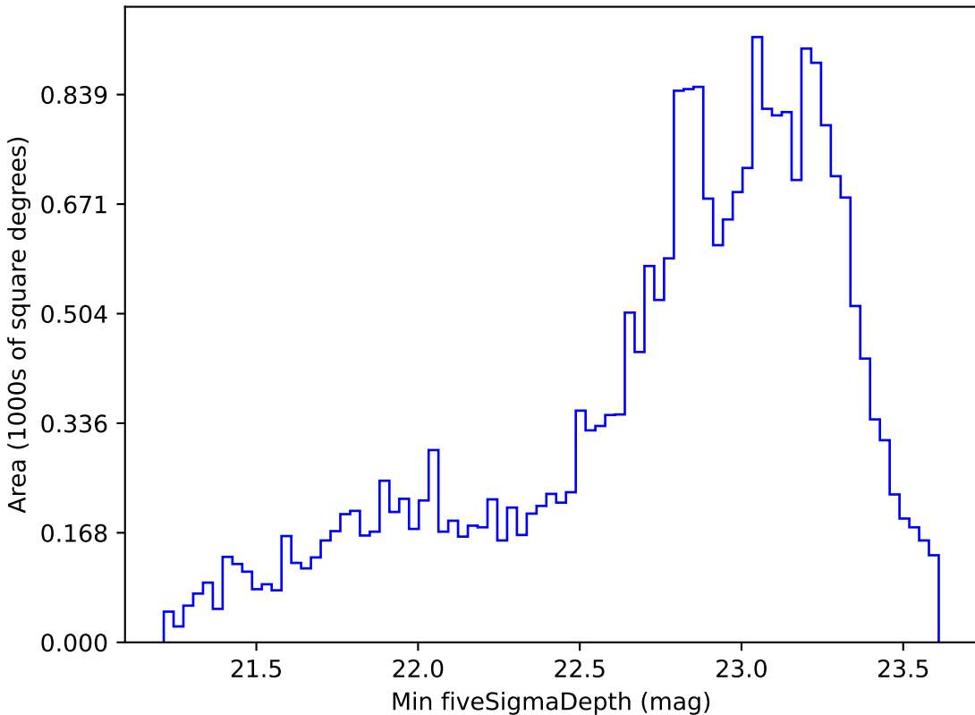
ddf_loaded_fl1_v3.4_10yrs Yr 1 i band: Min fiveSigmaDepth
