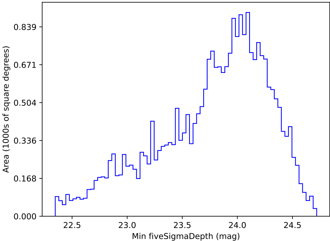
ddf_loaded_fl1_v3.4_10yrs Yr 1 g band: Min fiveSigmaDepth
