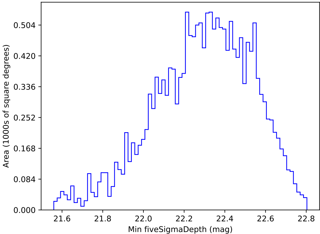
ddf_loaded_fl1_v3.4_10yrs WFD u band: Min fiveSigmaDepth
