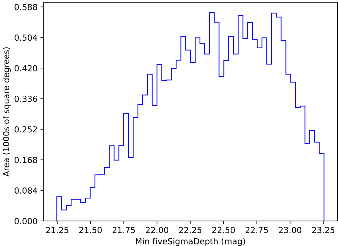
ddf_loaded_fl1_v3.4_10yrs WFD r band: Min fiveSigmaDepth
