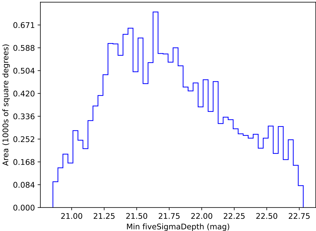
ddf_loaded_fl1_v3.4_10yrs WFD i band: Min fiveSigmaDepth
