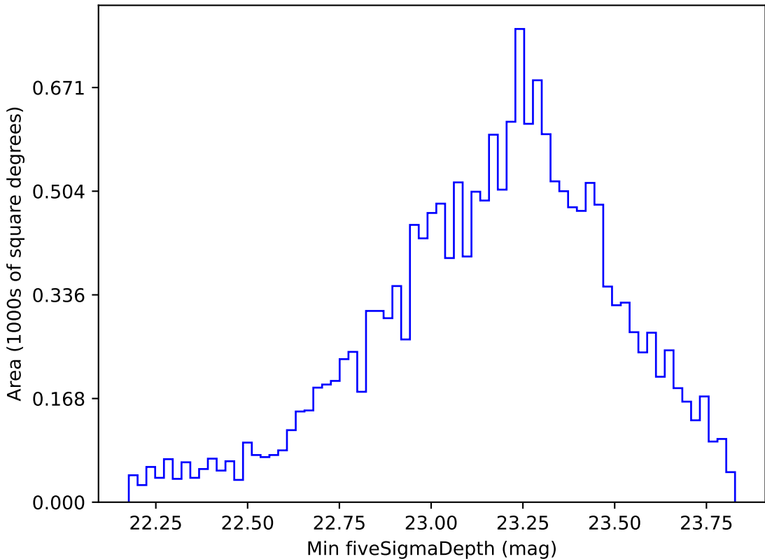
ddf_loaded_fl1_v3.4_10yrs WFD g band: Min fiveSigmaDepth
